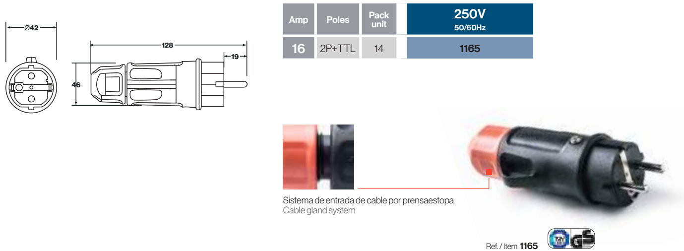
Base móvil con tapa goma / Mobile socket with rubber cover - Ref.Item 2165
