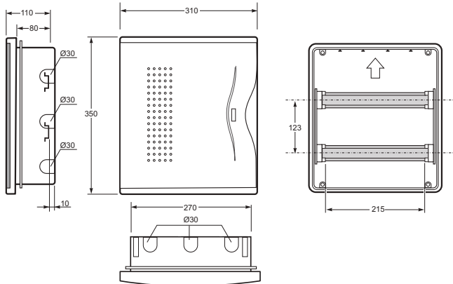
Armario / Enclosure - Ref. Item 3524 / 3724
