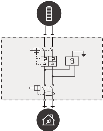
*Esquema Ref. E3SBDAC26-FVC125 *Ref. E3SBDAC26-FVC125 diagram
